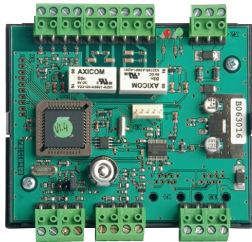
T-RS485 PCB
