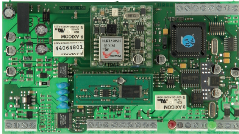
TELEN HOME CCU PCB
