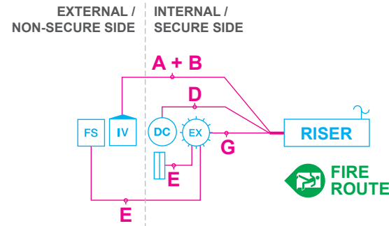
T N° 070/2A IPVIEW with EM24EX + DC + Fireman Switch
