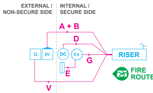
T No. 071/2A IPVIEW with EM24EX + DC + GERDA
