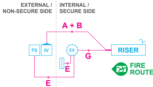
T N° 070/2 IPVIEW with EM24EX + Fireman Switch
