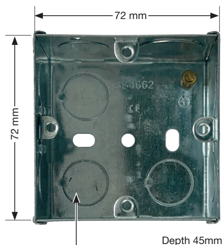
1 GANG (1G) FLUSH BACKBOX
