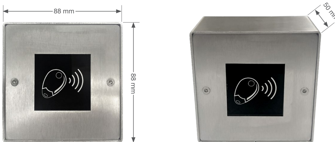
Surface mounted
